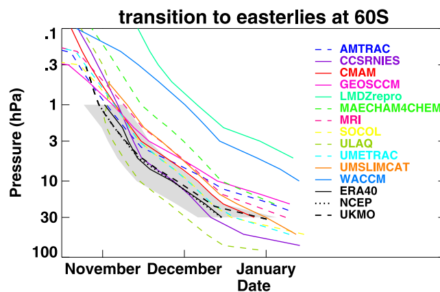
Figure 2. Descent of the zero zonal mean wind lines at 60°S based on the climatological mean annual cycle calculated from the monthly mean zonal winds. The grey area indicates the variation of the timing in the transition from westerlies to easterlies for ERA-40 due to a plus or minus one interannual standard deviation in the mean annual cycle. Tick marks refer to the first of the month, and climatological means are calculated as in Figure 1.
