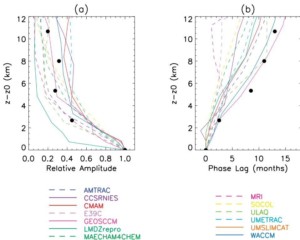
Figure 9. Vertical variation of (a) amplitude and (b) phase lag of annual cycle of water vapor averaged between 10^{\circ}\text{S} and 10^{\circ}\text{N} . The amplitude is normalized to unity and phase lag is set to zero at the level where the amplitude is maximum (between 16 and 20 km), which varies between the CCMs. The vertical axis in both plots is the distance from level of maximum amplitude. Solid circles are HALOE observations.
