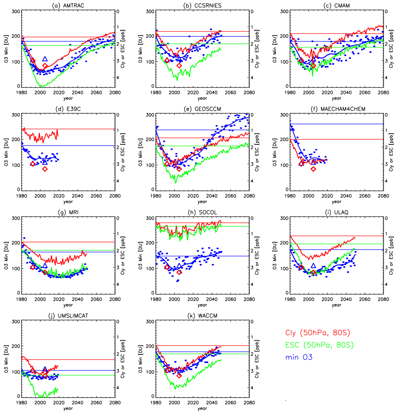
Figure 10. Daily minimum total column ozone (in DU) poleward of 60^{\circ}\text{S} for September–October with total inorganic chlorine ( \text{Cl}_y in ppb) and ESC ( \text{Cl}_y + 60\text{Br}_y in ppb) at 50 hPa for October at 80^{\circ}\text{S} superimposed. (a–k) Time series for the participating CCMs in alphabetical order. Triangles show observations for \text{Cl}_y and minimum ozone as in Figures 1c and 8b. For minimum ozone the blue circles show the individual years for each CCM and the solid lines show the smoothed curves as in Figure 8b. Horizontal lines indicate the 1980 values of the plotted quantities.
