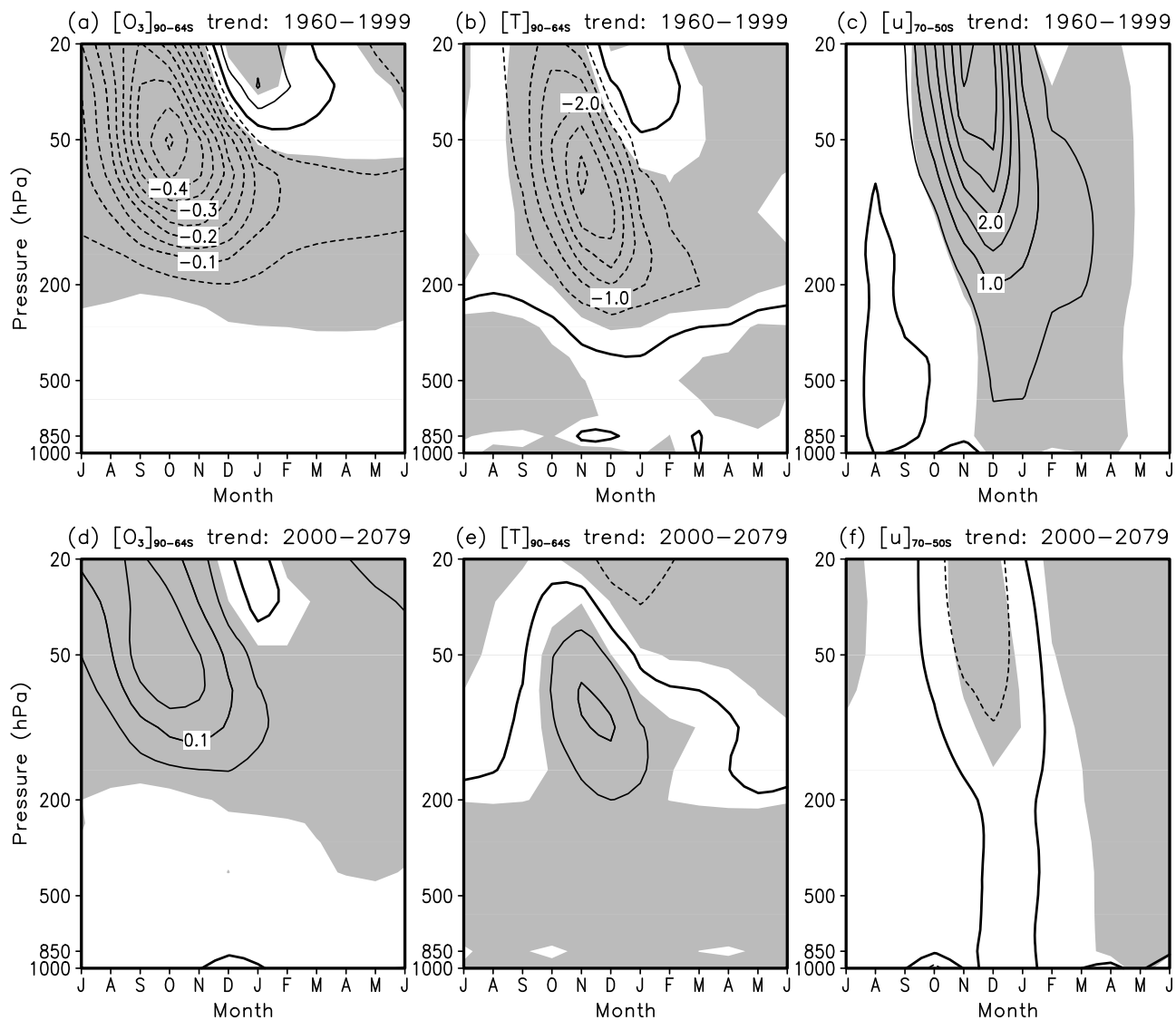
Figure 3. Linear trends of (a, d) the monthly mean [O_3] , (b, e) [T] integrated south of 64^\circ\text{S} , and (c, f) [u] integrated from 70^\circ to 50^\circ\text{S} . The multimodel mean trends are computed for the time period of 1960–1999 in the CCMVal-2 REF-B1 runs (Figures 3a–3c) and for the time period of 2000–2079 in the CCMVal-2 REF-B2 runs (Figures 3d–3f). Starting month in the x axis is July, and contour intervals are 0.05 ppmv/decade (Figures 3a and 3d), 0.5 K/decade (Figures 3b and 3e), and 0.5 \text{m s}^{-1} /decade (Figures 3c and 3f). Zero lines are denoted with thick black lines, and multimodel mean values exceeding 1 standard deviation are shaded.
